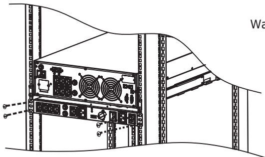
Chart 1: Rack mounting
