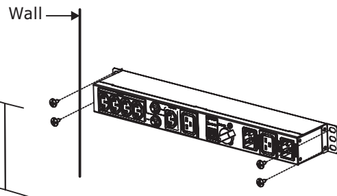
Chart 2: Wall mounting
