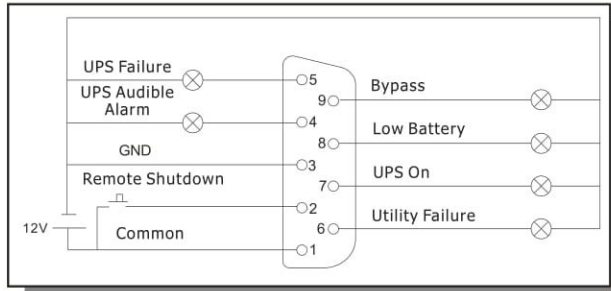
User Interface
