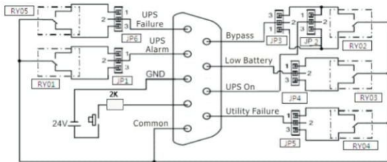
Fig 1 Pin definition and internal logical connection
