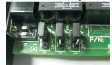
Fig. 7 Jumper setting for ACTIVE OPEN
