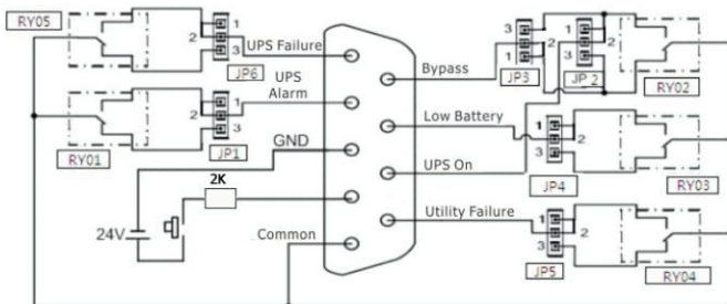
Fig 2 Connection for ACTIVE CLOSE
